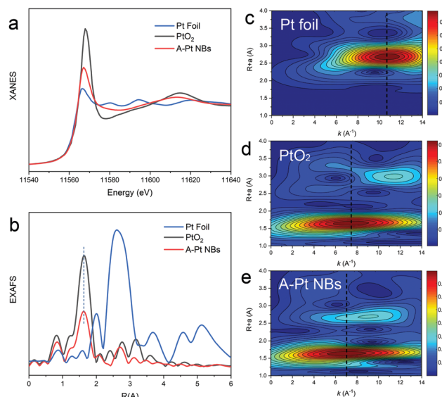
Fig. 3 X-ray absorption spectroscopic studies of the A-Pt NBs. (a) XANES spectra at the Pt \text{L}_3 -edge of the A-Pt NBs, \text{PtO}_2 , and Pt foil. (b) Fourier transform (FT) EXAFS spectrum of the A-Pt NBs compared with \text{PtO}_2 and Pt foil at the Pt \text{L}_3 -edge. (c–e) Wavelet transform (WT) EXAFS of the Pt foil (c), \text{PtO}_2 (d) and A-Pt NBs (e).
