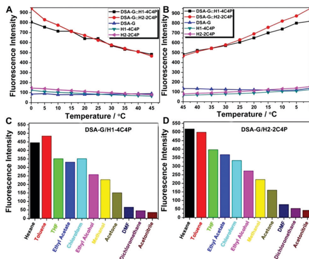
Fig. 2 Plots of fluorescence intensity changes of DSA-G⊂H1-4C4P and DSA-G⊂H2-2C4P (control experiments: individual H1-4C4P, H2-2C4P and DSA-G) at \lambda_{\text{em}} = 535 nm upon (A) elevating and (B) lowering the temperature ( \lambda_{\text{ex}} = 350 nm; slit widths: ex. 3 nm, em. 5 nm; 25 °C; concentrations: [H1-4C4P] = [H2-2C4P] = 35 \mu\text{M} , [DSA-G] = 70 \mu\text{M} ); histograms of fluorescent intensity changes of (C) DSA-G⊂H1-4C4P and (D) DSA-G⊂H2-2C4P influenced by solvents ( \lambda_{\text{ex}} = 350 nm; slit widths: ex. 3 nm, em. 5 nm; 25 °C; concentrations: [H1-4C4P] = [H2-2C4P] = 14 \mu\text{M} , [DSA-G] = 28 \mu\text{M} ; all the solvents are mixed with \text{CHCl}_3 at a volume ratio of 1:1 to guarantee the solubility).
