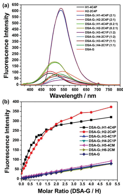
Fig. 1 (a) Fluorescence emission spectra ( \lambda_{\text{ex}} = 350 nm; slit widths: ex. 5 nm, em. 5 nm; 25 °C, [H1-4C4P] = 50 \mu\text{M} ; [H2-4C4P] = 50 \mu\text{M} ; [DSA-G⊂H1-4C4P] = 100 \mu\text{M} ⊂50 \mu\text{M} ; [DSA-G⊂H2-2C4P] = 100 \mu\text{M} ⊂50 \mu\text{M} ; [DSA-G⊂H1-4C4P] = 10 \mu\text{M} ⊂50 \mu\text{M} ; [DSA-G⊂H2-2C4P] = 10 \mu\text{M} ⊂50 \mu\text{M} ; [DSA-G⊂H3-4C1P] = 100⊂200 \mu\text{M} ; [DSA-G⊂H4-2C1P] = 100⊂200 \mu\text{M} ; [DSA-G⊂H3-4C1P] = 100⊂2100 \mu\text{M} ; [DSA-G⊂H4-2C1P] = 100⊂100 \mu\text{M} ; [DSA-G] = 100 M) and (b) changes of fluorescence emission intensity of DSA-G⊂H1-4C4P, DSA-G⊂H2-2C4P, DSA-G⊂H3-4C1P, DSA-G⊂H4-2C1P, H5-4CM/DSA-G, H6-2CM/DSA-G and DSA-G (data gathered from Fig. S20, ESI†).
