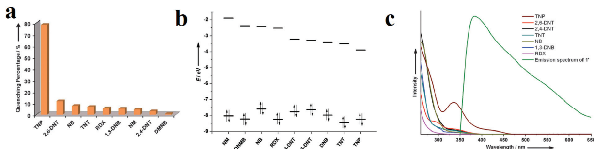
Fig. 4 Application of [Cd(NDC)_{0.5}(PCA)] \cdot G_x in the detection of TNP. (a) Percentage of fluorescence quenching obtained for different analytes at room temperature. (b) HOMO and LUMO energies for explosive analytes arranged in descending order of LUMO energy. (c) Spectral overlap between the absorption spectra of the analytes and the emission spectrum of the MOF in MeCN. Reproduced with permission from ref. 95.
