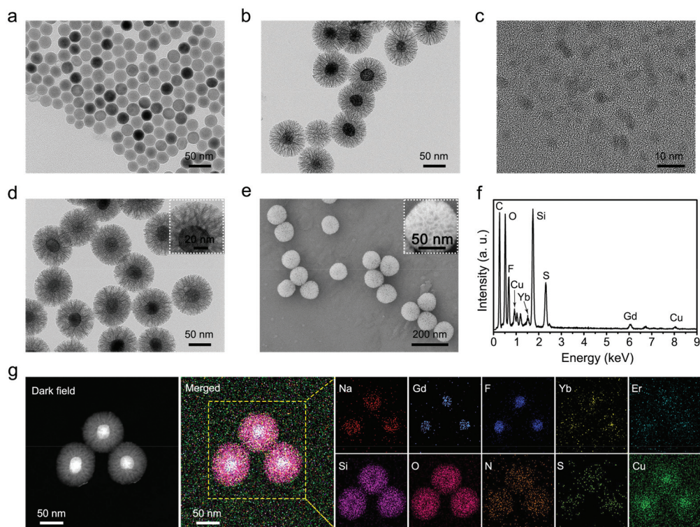
Fig. 1 Structural and compositional characterization of UMNOCC-PEG nanoparticles. TEM images of (a) the \text{NaGdF}_4:\text{Yb,Er} core nanoparticles, (b) \text{UCNP@MSN-SNO} , (c) \text{Cu}_2\text{O} nanodots, and (d) UMNOCC-PEG nanoparticles. (e) SEM image and (f) corresponding EDS spectrum of the UMNOCC-PEG nanoparticles. (g) Dark-field STEM image and the corresponding elemental mappings of UMNOCC-PEG nanoparticles.
