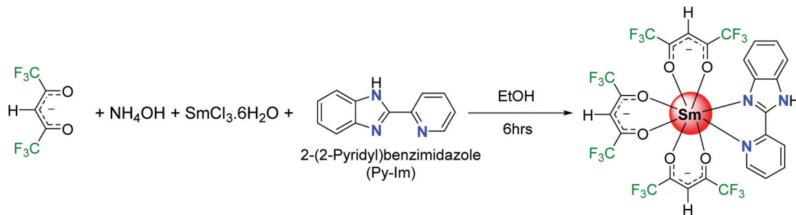
Scheme 1 Synthesis of [\text{Sm}(\text{hfaa})_3(\text{Py-Im})] complex.
