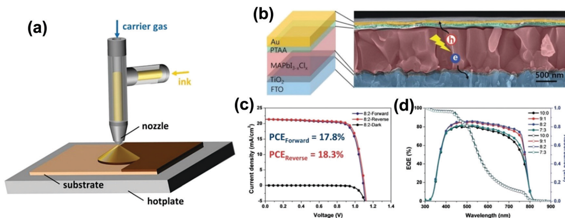
Fig. 6 Spray coating. (a) Schematic of the spray coating process. (b) SEM cross-sectional image of a high-quality spray-coated MAPb 1-x Cl x perovskite absorber. (c) PCEs up to 18.3% in reverse J - V characteristics and (d) high external quantum efficiency (EQE) were achieved, which is a result of a careful solvent engineering of the spray process. Reproduced with permission from ref. 91. Copyright © 2019 WILEY-VCH.
