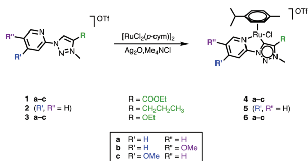
Scheme 1 Synthesis of 1,2,3-triazolyldiene ruthenium(II) complexes 4–6 .
