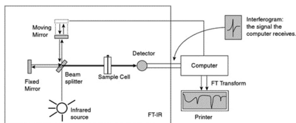
Fig. 1 Schematic diagram by Pavia et al. 10 of an FTIR instrument. From Pavia/Lampman/Kriz/Vyvyann. Introduction to Spectroscopy, 4E. © 2009 Brooks/Cole, a part of Cengage, Inc. Reproduced by permission. http://www.cengage.com/permissions .
