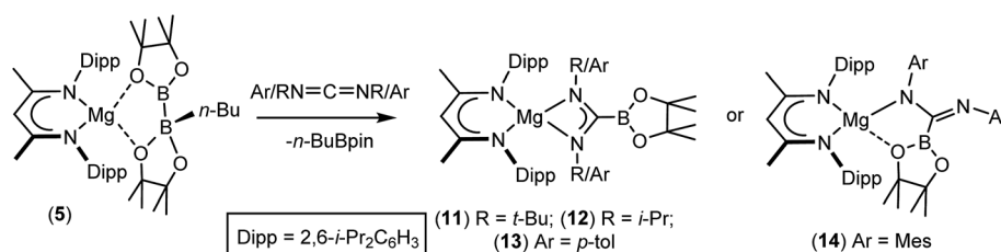
Scheme 3 Synthesis of compounds 11–14 .
