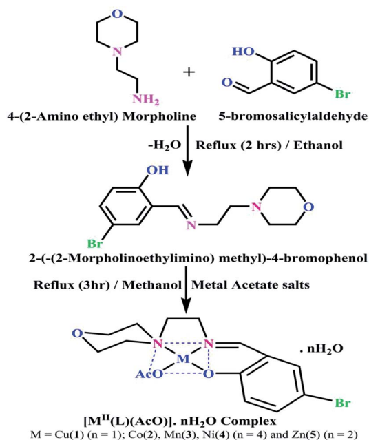
Scheme 1 The proposed structure of complexes 1–5 [M^{II}(L)(AcO)] \cdot nH_2O .
