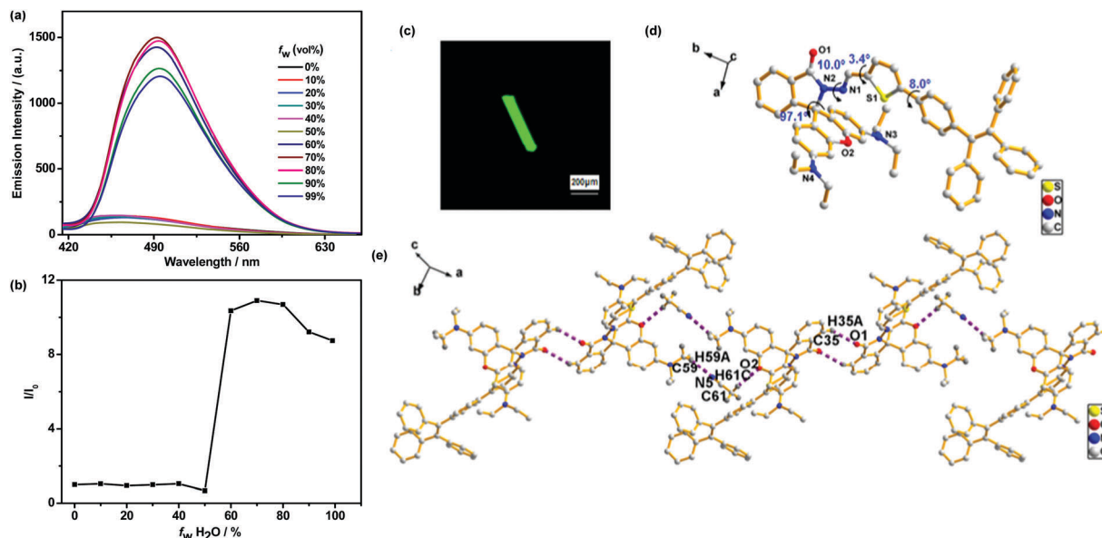
Fig. 1 (a) Fluorescence spectra of TPETHRB (10 \mu M) in CH 3 CN-H 2 O solution with different water fractions ( f_w ). (b) Plot of ( I/I_0 ) vs. f_w , where I_0 and I are the emission intensities of TPETHRB in CH 3 CN and CH 3 CN-H 2 O mixture. (c) Confocal laser scanning image. (d) Single-crystal structure of TPETHRB (CCDC 1814395) and (e) chain crystallography diagram.† TPETHRB single crystal was incubated in CH 3 CN solution and crystallographic data were collected at 296 K.
