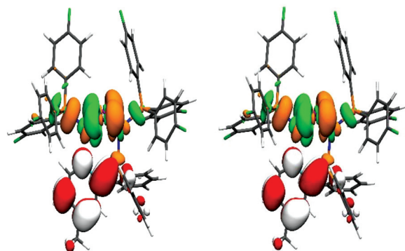
Fig. 7 Natural transition orbitals of Cu-2b for the lowest singlet (left) and triplet (right) excitation at the T_1 structure. The colours green/orange indicate the hole while red/white correspond to the electron. (Isovalue: \pm 0.03a_0^{-3/2} , Cu = blue, P = orange, I = purple, N = cyan, F = green, C = grey, H = white).
