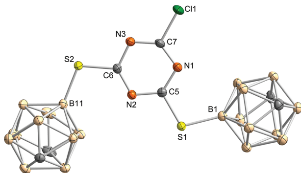
Fig. 2 Molecular structure of 2-chloro-4,6-bis(1,7-dicarba-closo-dodecaboran-9-ylthio)-1,3,5-triazine (3). Hydrogen atoms are omitted for clarity. Thermal ellipsoids are drawn at the 50% level of probability. Selected bond lengths, distances (pm) and bond angles ( ^{\circ} ): Cl1–C7 172.7(2), S1–C5 174.2(2), S2–C6 173.4(2), S1–B1 187.2(2), S2–B11 185.9(2), \diamond ...N1 0.4, \diamond ...C5 1.5, \diamond ...N2 1.2, \diamond ...C6 0.0, \diamond ...N3 1.0, \diamond ...C7 0.9, \diamond ...S1 4.9, \diamond ...S2 4.3, \diamond ...Cl1 3.8, \diamond ...B1 41.0, \diamond ...B11 1.2; C5–S1–B1 106.1(1), C6–S2–B11 107.6(1); \diamond represents the mean plane of the triazine core, formed by N1, C5, N2, C6, N3 and C7.
