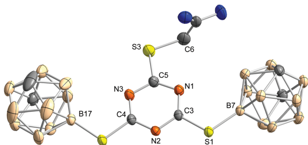
Fig. 3 Molecular structure of 2-([4,6-bis(1,7-dicarba-closo-dodecaboran-9-ylthio)-1,3,5-triazine-2-yl]thio)acetic acid (4) obtained from methanol. Thermal ellipsoids are drawn at the 50% level of probability. The acid and the methyl ester co-crystallise in a ratio of 0.678(7):0.322(7). Here, only the acid is shown. Hydrogen atoms and co-crystallised methanol molecules are omitted for clarity. Selected bond lengths, distances (pm) and bond angles ( ^{\circ} ): S1–C3 174.4(2), S1–B7 186.2(2), S2–C4 174.2(2), S2–B17 186.3(3), S3–C5 173.8(2), S3–C6 177.7(3), \diamond ...N1 0.8, \diamond ...C3 0.1, \diamond ...N2 0.6, \diamond ...C4 0.7, \diamond ...N3 0.0, \diamond ...C5 0.8, \diamond ...S1 2.0, \diamond ...S2 2.2, \diamond ...S3 8.5, \diamond ...B7 13.0, \diamond ...B17 16.7, \diamond ...C6 27.9, C3–S1–B7 109.9(1), C4–S2–B17 107.0(1), C5–S3–C6 103.5(1); \diamond represents the mean plane of the triazine core, formed by N1, C3, N2, C4, N3 and C5.
