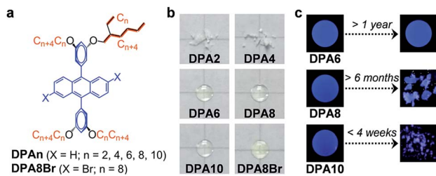
Fig. 1 (a) Chemical structures of DPA n ( n = 2, 4, 6, 8, \text{ and } 10 ) and DPA8Br. (b) Photographs of freshly synthesized DPA n and DPA8Br in daylight at 20 °C, with a drop of fluid or powder of solid on a glass plate. (c) Photographs of DPA 6 , DPA 8 , and DPA 10 as fresh (left) and after long-term of aging at ambient temperature (right) taken under irradiation of a UV lamp (365 nm).
