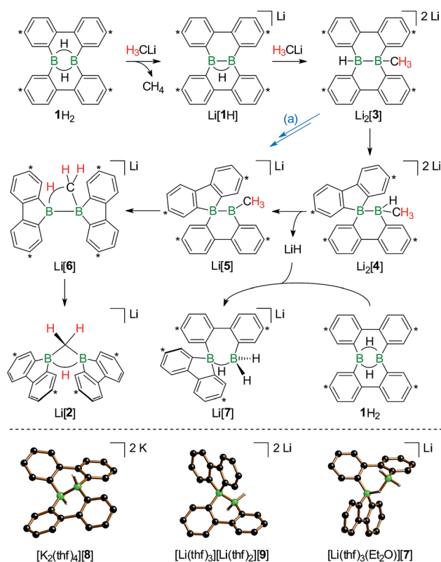
Scheme 5 Proposed reaction mechanism explaining the formation of Li[ 1H ], Li[ 2 ], and Li[ 7 ] from an equimolar mixture of H 3 CLi and 1H 2 (top; carbon atoms marked with asterisks bear tBu substituents). The alternative pathway (a) leads from Li[ 2 ] to Li[ 5 ], first via hydride elimination and second via a 1,2-phenyl shift. Molecular structures of [K 2 (thf) 4 ] 8 , [Li(thf) 3 ][Li(thf) 2 ] 9 , and [Li(thf) 3 (Et 2 O)] 7 in the solid state (bottom). The solvent-separated cations, all tBu groups, and all CH atoms are omitted for clarity.
