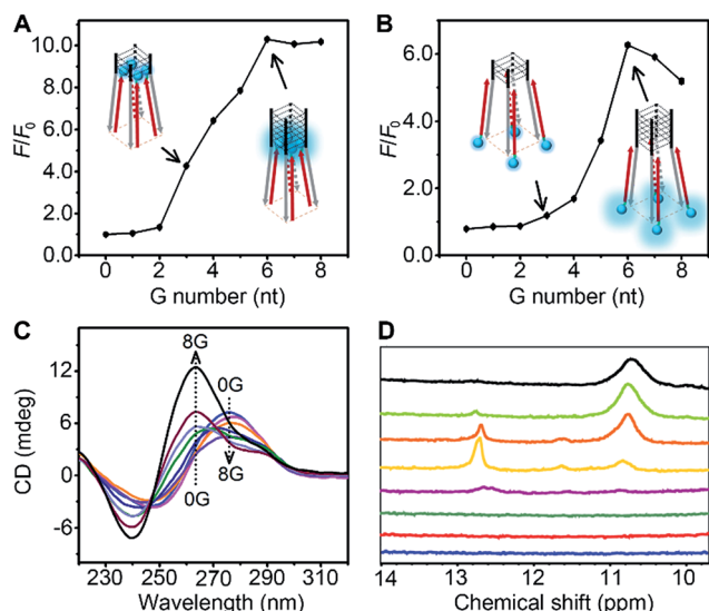
Fig. 4 Ratios of fluorescence peak intensity of (A) 1.0 \mu M O1-DTPE and (B) O1'-DTPE after and before ( F/F_0 ) hybridization with O1'- n G ( n = 0 to 8) in TE reaction buffer at 25 °C. (C) CD spectra of 20 \mu M O1'- n G ( n = 0 to 8) in TE reaction buffer at 25 °C. (D) 1 H-NMR spectra of O1'- n G ( n = 1 to 8 from bottom to top) in 10 mM phosphate buffer pH 7.4, with 100 mM NaCl and 10 mM MgCl 2 at 25 °C.
