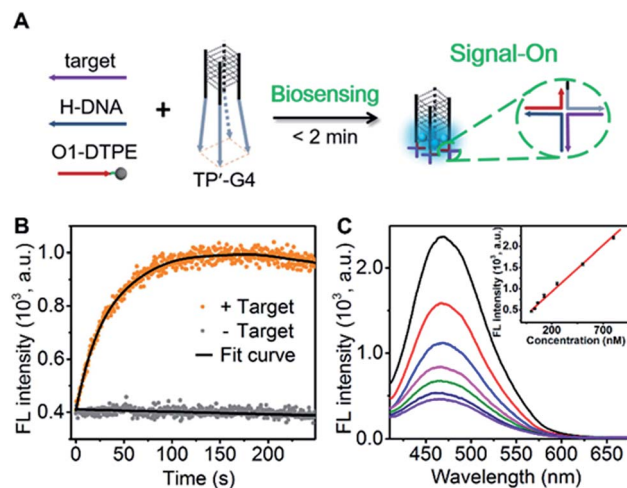
Fig. 7 (A) Schematic illustration of the DNA detection strategy that relies on the self-assembly of four-way junctions. (B) Time-dependent fluorescence signal for 1.0 \mu M O1'-DTPE, 1.0 \mu M H-DNA, and 1.0 \mu M TP'-G4-5 bp in the presence and absence of target DNA in TE reaction buffer at 25 ^{\circ} C. (C) Fluorescence spectra of 1.0 \mu M O1'-DTPE after mixing with 1.0 \mu M H-DNA and TP'-G4 in the presence of target DNA at different concentrations for 1.5 min in TE reaction buffer at 25 ^{\circ} C. Inset is the calibration curve.
