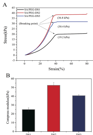
Fig. 4 (A) The stress–strain curves of SA/PEG hydrogels by a linear 1 \text{ N min}^{-1} ramp force loading to test the breakage strength. (B) The compressive modulus of the SA/PEG hydrogels.
