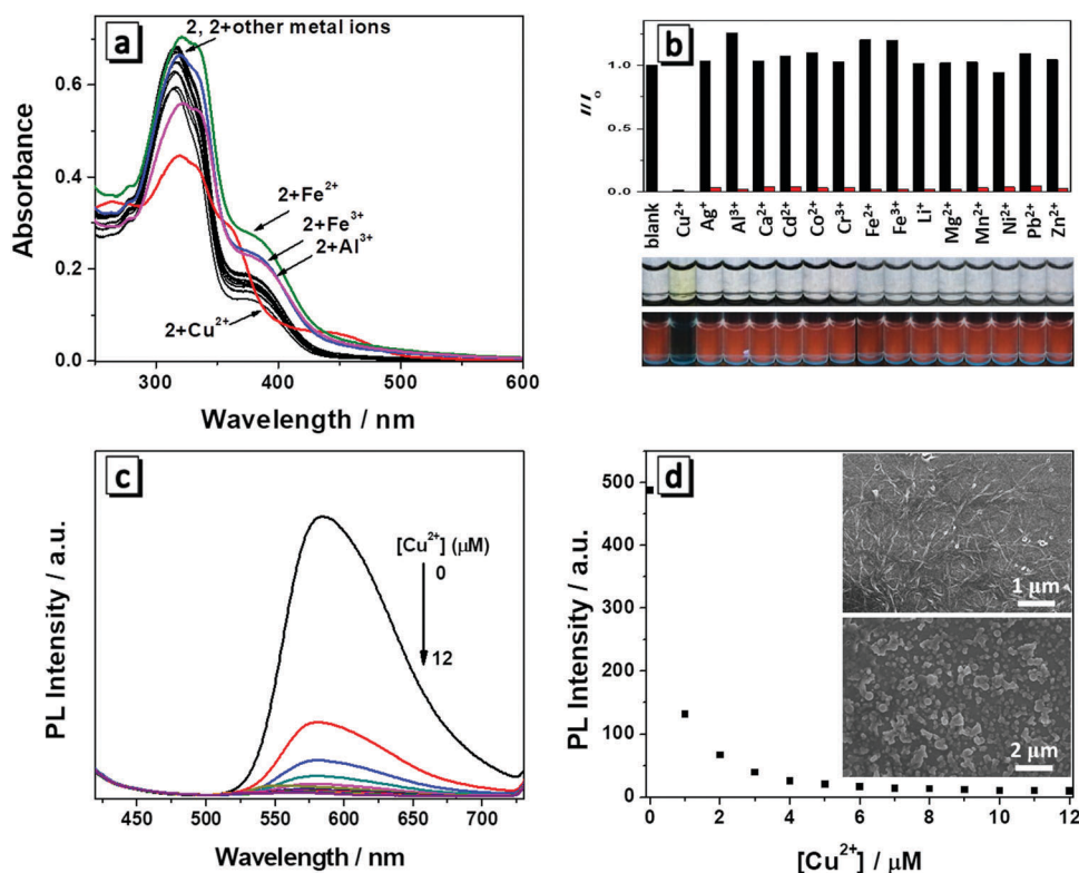
Fig. 5 (a) UV spectra of 2 (10 μM) upon the addition of various metal cations (10 μM) in THF/ \text{H}_2\text{O} (1/9, v/v); (b) variation of the fluorescence intensity at 586 nm ( \lambda_{\text{ex}} = 380 nm) of 2 (10 μM) after addition of various metal cations. Black bars represent the addition of different metal ions (10 μM) to the solution of 2 , whereas the red bars represent the subsequent addition of \text{Cu}^{2+} (10 μM) to the solution containing a specific metal ion (the concentration of \text{Li}^+ , \text{Mg}^{2+} and \text{Ca}^{2+} was 1 mM, \text{Al}^{3+} , \text{Fe}^{2+} and \text{Fe}^{3+} was 10 μM, other transition metal ions was 100 μM); the photographs show 2 (10 μM) upon addition of 1 equiv. of various metal ions in THF/ \text{H}_2\text{O} (1/9, v/v) taken under natural light (upper) and UV light (lower). (c) Fluorescence titration spectra of 2 (10 μM) with 0–12 μM \text{Cu}^{2+} ; (d) the plot of fluorescence intensity at 586 nm versus \text{Cu}^{2+} concentrations; insets: SEM images of 2 (10 μM) in the absence (upper) and presence (lower) of 1 equiv. of \text{Cu}^{2+} in THF/ \text{H}_2\text{O} (1/9, v/v).
