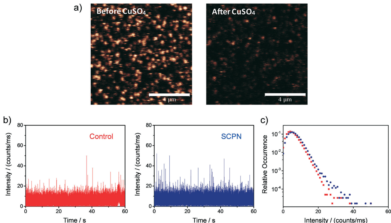
Fig. 8 Representative single-SCP activity measurement. a) Confocal images ( 10 \times 10 \mu\text{m} ) showing the Alexa Fluor 488-labeled and biotin-functionalized SCPNs immobilized on a streptavidin-functionalized glass coverslip before (left) and after (right) the addition of \text{CuSO}_4 . The bar in the panel represents 4 \mu\text{m} . b) Fluorescent intensity time traces and c) corresponding intensity distributions obtained when binning the data with 1 ms bin size. The data was recorded on the location of one individual SCPN (blue) and on an empty area on the surface (red; control).
