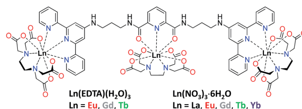
Fig. 1 Structural formula of multidentate tdt ligand composed of dpa and two tpy units free for binding \text{Ln}(\text{EDTA}) \cdot (\text{H}_2\text{O})_3 or \text{Ln}(\text{NO}_3)_3 \cdot 6\text{H}_2\text{O} .
