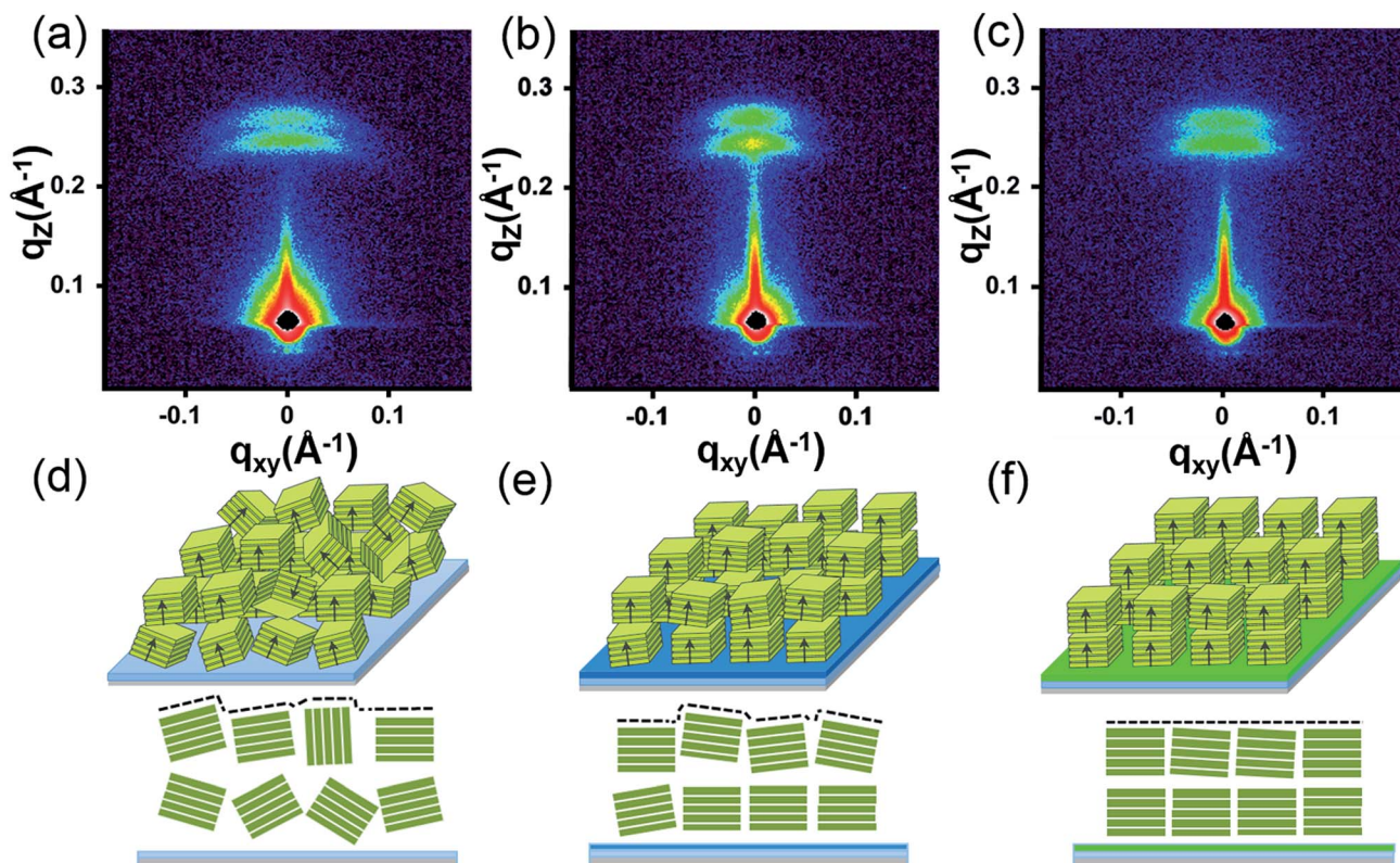
Fig. 4 (a)–(c) GISAXS pattern of SA-Bu evaporated on ITO, PPA-IITO and OPA-IITO substrates and (d)–(f) the proposed crystallite stacking models, respectively.
