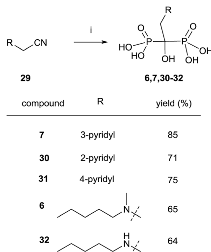
Scheme 9 Reagents and conditions: (i) \text{CH}_3\text{SO}_3\text{H} , 8 h, 100 °C; then \text{PCl}_3 , 70 °C, 5 h; then \text{H}_2\text{O} , 15 h, 98 °C.
