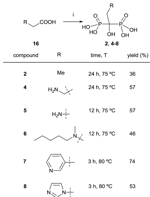
Scheme 7 Reagents and conditions: (i) \text{PCl}_3 (3.2 equiv.), \text{MeSO}_3\text{H} , see scheme for time and temperature; then \text{H}_2\text{O} , 4–5 h, 105 °C; then 50% aq. \text{NaOH} to \text{pH} = 1.8\text{--}2.0 .
