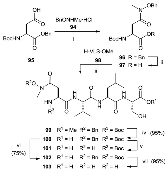
Scheme 25 Reagents and conditions: (i) CD1, i\text{Pr}_2\text{NEt} . (ii) 1 N NaOH, MeOH, (iii) EDC, HOBT, i\text{Pr}_2\text{NEt} , HVLS-OMe, (iv) \text{Na}_2\text{CO}_3 (1.0), 2 : 1 MeOH, \text{H}_2\text{O} . (v) \text{H}_2 , 10% Pd/C, MeOH. (vi) Anhydrous HCl/dioxane, EtOAc. (vii) \text{H}_2 , 10% Pd/C, MeOH.
