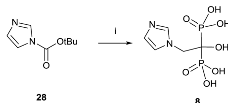
Scheme 8 Reagents and conditions: (i) \text{H}_3\text{PO}_3 , 4-chlorobenzene, 25 °C, 15 min; then \text{CH}_3\text{SO}_3\text{H} , 30 min, 70 °C; then \text{POCl}_3 , 95 °C, 24 h; then \text{H}_2\text{O} , 6 h, 90 °C; then 30% NaOH, pH = 4.1.
