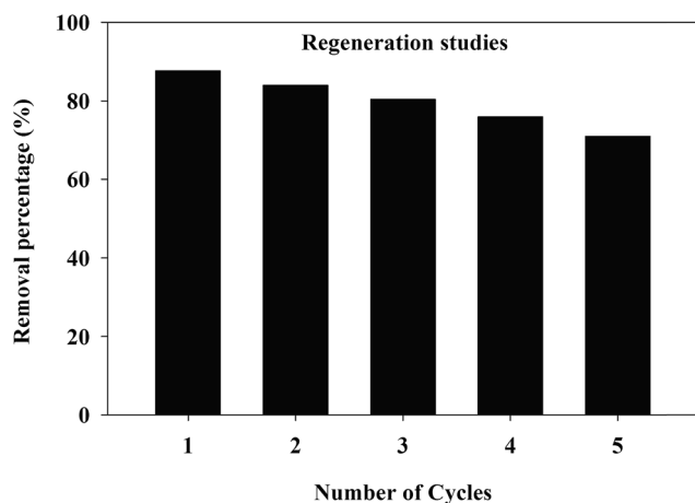
Fig. 13 Desorption–regeneration experiment of the TW/Fe 3 O 4 composite for Cr(vi) removal.
