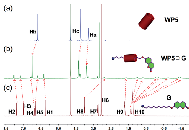
Fig. 3 Partial 1 H-NMR (400 Hz, D 2 O, 293 K) spectra: (a) WP5 (10.0 mM); (b) WP5 (10.0 mM) and G (10.0 mM); (c) guest molecule G (10.0 mM).
