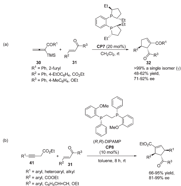
Scheme 19 The catalytic asymmetric Lu's [3 + 2] cycloadditions developed by Loh's group.
