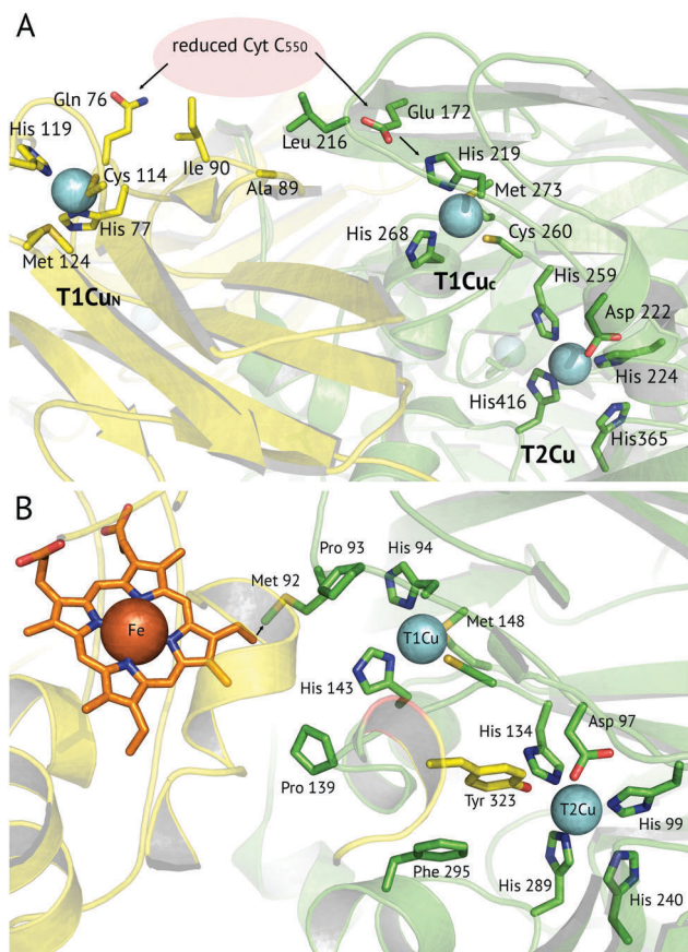
Fig. 6 Proposed electron transfer routes between the redox centres of 3-domain CuNiRs. In (A) HcNiR the external electron donor partner protein cyt. C 550 is proposed to bind to a hydrophobic patch spanning the N-terminal (near Ala89, Ile90) and cupredoxin domains (near Leu216), where it is positioned for electron transfer to both the T1Cu N and T1Cu C sites (indicated by arrows). 74 In (B) RpNiR , the proposed internal electron transfer route is from the haem (CBC atom) to Met92 and to the T1Cu site. 75 Interface and T2Cu water molecules have been omitted from the figures for clarity.
