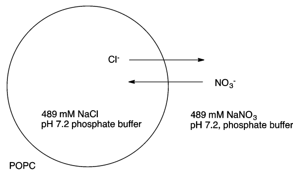
Fig. 14 Anion transport experiments with compounds 53–74.
