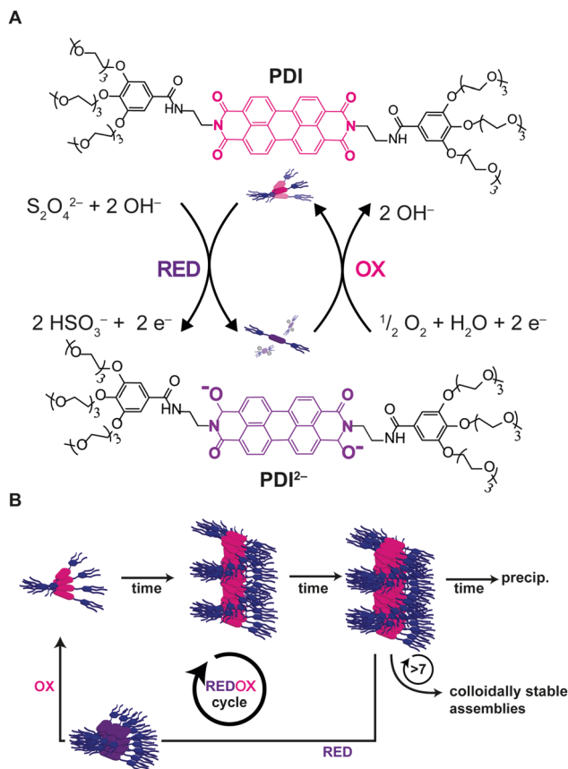
Fig. 12 Chemical fuels. (A) PDI was reduced upon addition of dithionite to the dianion PDI^{2-} , upon exposure to air PDI^{2-} is oxidized back to the neutral PDI. (B) The number and frequency of redox cycles will affect the outcome of the assemblies due to progressive changes in the assemblies after each redox cycle. Adapted from ref. 49 with permission from The Royal Society of Chemistry.
