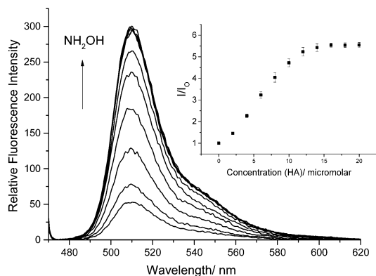
Fig. 1 Fluorescence changes observed for probe 1 ( 0.5 \mu\text{M} ) during the addition of HA ( 0 – 20 \mu\text{M} ), in 1% DMSO PBS Buffer at pH 7.4. \lambda_{\text{ex}} = 465 \text{ nm} , with a 5 min delay between additions of HA. Inset: Relative fluorescence changes ( I/I_0 ) as a function of HA concentration ( 0 – 20 \mu\text{M} ).
