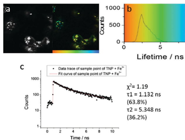
Fig. 4 Two-photon FLIM of [\text{TNPH}]^+ (showing the same cluster of HeLa cells as above, albeit with slightly shifted field of view due to instrument alignment) formed from TNP in the presence of excess aqueous \text{FeCl}_3 (37 °C, 50 \mu\text{M} , 1% DMSO, 15 minutes incubation, 1% DMSO of TNP , 5 eq. \text{FeCl}_3 ). Images show: (a) 2P fluorescence lifetime FLIM map ( \lambda_{\text{ex}} = 810 nm); (b) corresponding lifetime distribution curve (ns) showing an average lifetime distribution ( \tau_m ) of 2.40 \pm 1.25 ns, (c). A representative point decay trace corresponding to the blue cursor whereby the value of the \tau_2 component (ca. 5 ns, similar to the lifetime of free TNP in solution) is suggestive of a TNP core present within the lysosomal cells' regions (ESI†).
