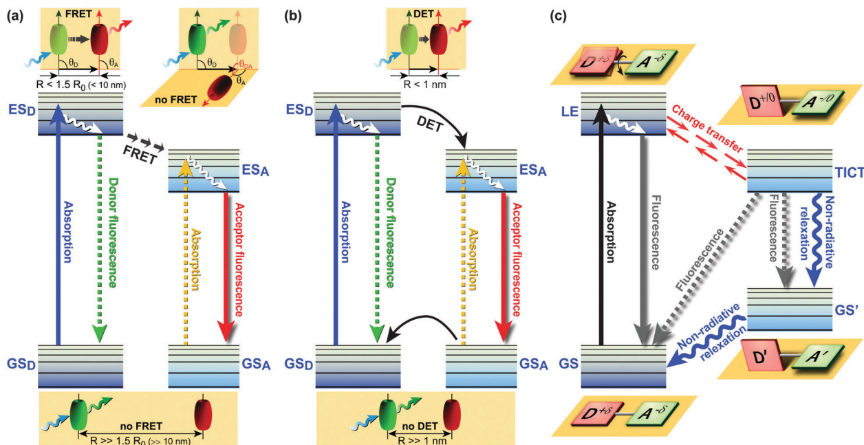
Fig. 1 Jablonski diagrams of various energy/electron donor-acceptor (D-A) systems. (a) Förster Resonance Energy Transfer (FRET); (b) Dexter Energy Transfer (DET); (c) Twisted Intramolecular Charge Transfer (TICT) dynamics. 11 Upon excitation from the GS, the LE state equilibrates rapidly with the TICT state after fast charge transfer. GS = ground state; GS D = ground state donor; GS A = ground state acceptor; ES D = excited singlet state donor; ES A = excited singlet state acceptor; LE = locally excited state; R = effective D-A distance.
