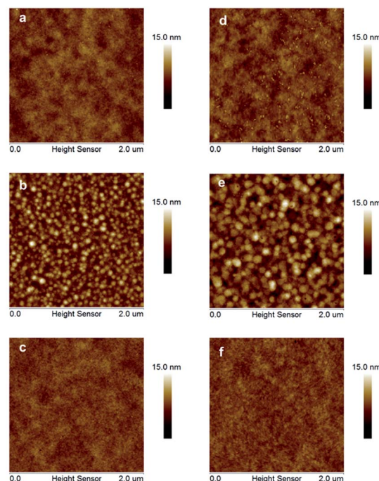
Fig. 6 AFM morphology images ( 2 \mu\text{m} \times 2 \mu\text{m} ). (a) PDTPPO-IDT pure film, RMS: 0.88 nm. (b) PDTPPO-IDT : PC 71 BM blend film without DIO, RMS: 1.62 nm. (c) PDTPPO-IDT : PC 71 BM blend film with 3% DIO, RMS: 0.68 nm. (d) PDTPPO-IDTT pure film, RMS: 0.99 nm. (e) PDTPPO-IDTT : PC 71 BM blend film without DIO, RMS: 1.87 nm. (f) PDTPPO-IDTT : PC 71 BM blend film with 3% DIO, RMS: 0.72 nm.
