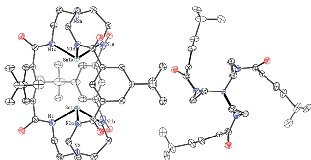
Fig. 1 Solid-state structure of [Sn 2 (mBDCA-5t)] 2- (1) with thermal ellipsoids (drawn using PLATON 17 ) shown at the 50% probability level and with [K(Kryptofix 2,2,2)] + cations, disorder, and hydrogen atoms omitted for clarity. Selected interatomic distances (Å) and angles (°): Sn1–N1 3.116(3), Sn1–N2 2.2531(16), Sn1–Sn1a 3.5373(7), N1–Sn1–N1a 100.82(5).
