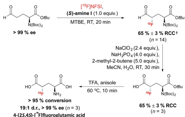
Scheme 7 Organomediated radiosynthesis of ^{18}\text{F} [(2 S ,4 S )-4- \text{F} ]-GLU. \dagger RCC determined by radio-HPLC relative to ^{18}\text{F} -NFSI.
