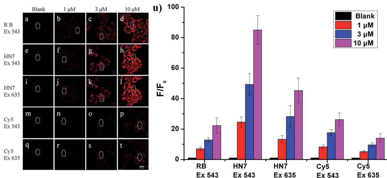
Fig. 5 Confocal fluorescence images of HeLa cells incubated with various dyes at 37 ^{\circ}\text{C} for 60 min (from left to right: 0, 1, 3, 10 \mu\text{M} ): (a–d) excitation at 543 nm for red emission of rhodamine B (560–630 nm); (e–h) excitation at 543 nm for red emission of HN7 (650–720 nm); (i–l) excitation at 635 nm for red emission of HN7 (650–720 nm); (m–p) excitation at 543 nm for red emission of Cy5 (650–720 nm); (q–t) excitation at 635 nm for red emission of HN7 (650–720 nm). Scale bar = 30 \mu\text{m} . (u) Relative fluorescence intensity obtained from the selected ellipse region of (a–t), respectively, averaged and plotted as a ratio to blank (a, e, i, m, q).
