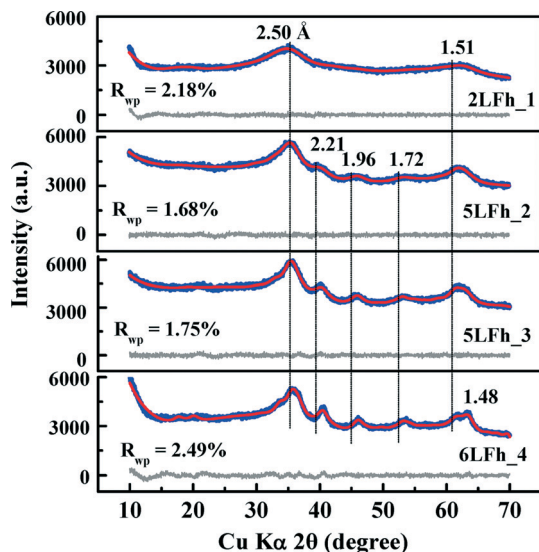
Fig. 1 XRD patterns of the four ferrihydrite samples (blue lines), Rietveld fitting results (red solid lines), and difference between the experimental data and the fit (black solid lines below the data). R_{wp} is the goodness of fit.
