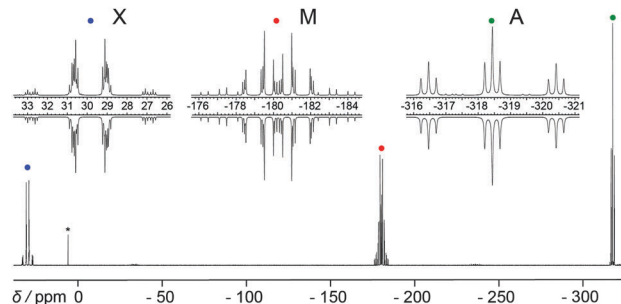
Fig. 18 ^{31}P\{^1H\} NMR spectrum of the butterfly-shaped dication 105 ^{2+} (upwards) and simulation (downwards). This figure has been reproduced from Angewandte Chemie with permission from John Wiley and Sons. 129
