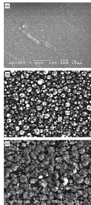
Fig. 24 SEM of films grown from AACVD deposition of \text{InMe}_3 and MeOH at (a) 400^\circ\text{C} ; (b) 450^\circ\text{C} ; and (c) 500^\circ\text{C} . Reproduced with permission from ref. 176 Copyright 2013 Royal Australian Chemical Institute.
