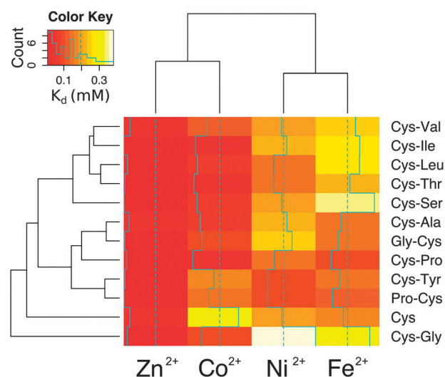
Fig. 4 Heatmap and clustering based on the Euclidean distances of the K_d values of the metallopeptides. Cys and Cys-Gly behave differently than the rest of the peptides. Excluding Cys and Cys-Gly, the peptides can be divided into two groups: one group with lower affinity for \text{Fe}^{2+} (Cys-Val, Cys-Ile, Cys-Leu, Cys-Thr, Cys-Ser) and one group with higher affinity for \text{Fe}^{2+} (Cys-Ala, Gly-Cys, Cys-Pro, Cys-Tyr, Pro-Cys).
