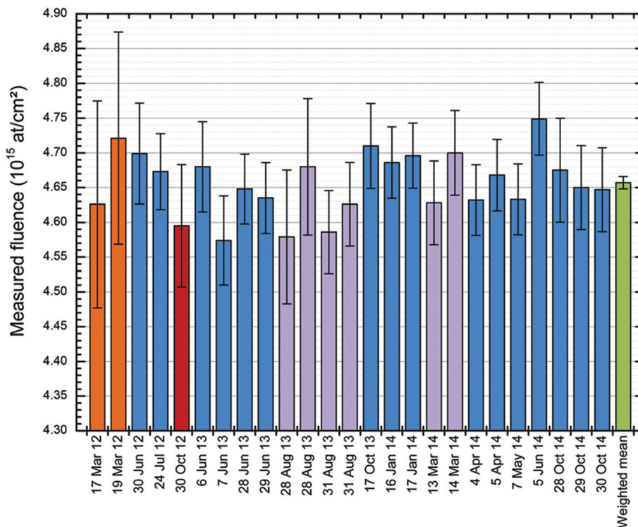
Fig. 5 RBS repeatability. Repeated independent measurements of the retained ^{75}\text{As} dose in the sample measured by Jeaynes, Barradas & Szilágyi. 73 25 independent fluence measurements of the same sample by RBS over a 31 months period using various incident beams: 9 MeV ^{12}\text{C}^{4+} (in orange); 4 MeV ^7\text{Li}^{2+} (in red); 2 MeV ^7\text{Li}^{2+} (in purple) and 1.5 MeV ^4\text{He}^+ (in blue). The error bars are given for each measurement as the “Total combined standard uncertainty”. The weighted mean of the measurements (in green) has a precision (standard error on the mean) of 0.19%. The dataset has a standard deviation of 0.93%. ANOVA shows repeatability (the between-bottle variation, in ISO Guide 35 terms) of 0.33%. Reproduced from Fig. 7 of Colaix et al. , Analyst , 2015 87 with permission from the Royal Society of Chemistry (RSC).
