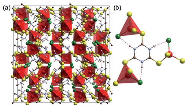
Fig. 1 Crystal structure of [\text{CuCl}(\text{ttcH}_3)] . 13 (a) 2 \times 2 \times 2 cells. (b) Connectivity of \text{CuCl}_3 tetrahedral with the thioctonitrile form of tri-thiocyanuric acid molecules (red: Cu, green: Cl, yellow: S, blue: N, brown: C, and white: H). Dotted lines show hydrogen bonding.
