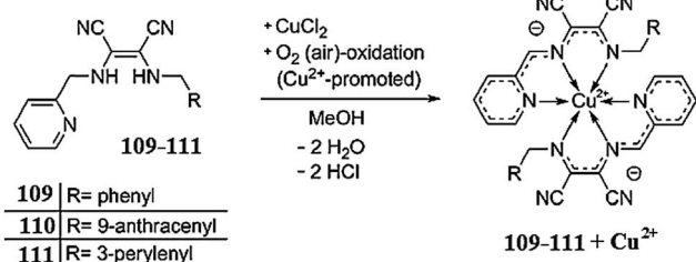
Fig. 94 Chemical structure of receptor 109–111 and selective \text{Cu}^{2+} -promoted air oxidation and deprotonation in the receptors to form copper complexes.
