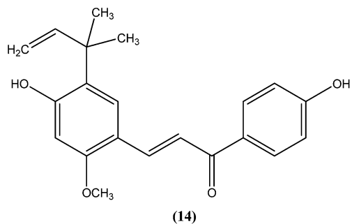
Licochalcone A
