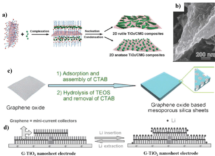
Fig. 109 Examples of 2d nanocomposites based on GRMs. (a) Assembly steps for a \text{TiO}_2/\text{GO} nanocomposite from SDS-modified graphene sheets. (b) SEM image of a rutile \text{TiO}_2/\text{GO} nanocomposite. (c) Fabrication process for GO based mesoporous silica sheets through the hydrolysis of tetraethylorthosilicate (TEOS), with cationic surfactant cetyl trimethylammonium bromide (CTAB)-functionalized GO as the template. (d) Lithium insertion and extraction in GMR sheets, where graphene acts as mini-current collectors during discharge and charge processes, facilitating the rapid diffusion of electrons during cycling processes. 2144
