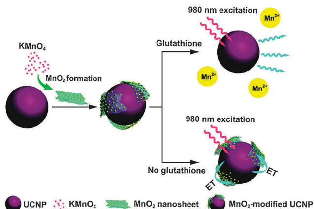
Fig. 19 Design and function of a glutathione (GSH) sensitive probe based on UCNP. The emission of the UCNP is quenched by the manganese oxide (MnO 2 ) nanosheets formed on the nanoparticle surface. The analyte GSH reduces MnO 2 , removes the nanosheets, and restores the emission of the UCNP. Reprinted with permission from ref. 37. Copyright © 2011, American Chemical Society.
