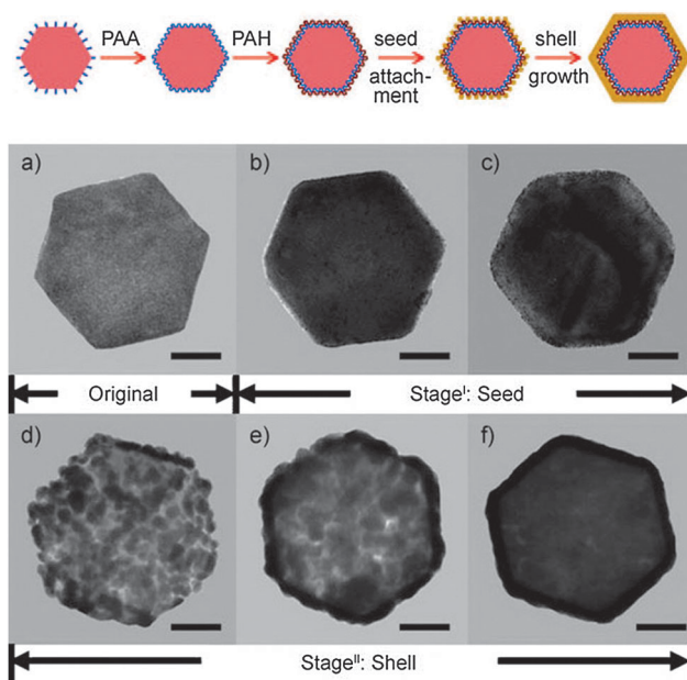
Fig. 20 Upper scheme: surface functionalization, attachment of gold nanoparticles, and growth of a gold nanoshell on an UCNPs. Lower TEM images of UCNP during gold seed attachment and shell growth, (a) original, (b and c) with increasing number of attached gold nanoparticles and (d–f) with growing gold nanoshells (scale bar: 50 nm). Reprinted with permission from ref. 125 Copyright © 2010, Wiley.
