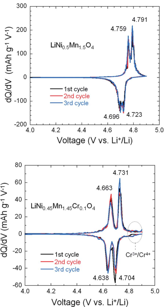
Fig. 11 Differential capacity curves, dQ/dV vs. V , of the un-doped LNM (top) and \text{LiNi}_{0.45}\text{Mn}_{1.45}\text{Cr}_{0.1}\text{O}_4 (bottom). The values at the peaks are given in volt. Reproduced with permission. 64
