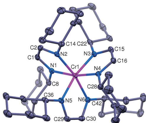
Fig. 1 The structural diagram of the [(\text{HLY})_3\text{Cr}]^+ cation ( \mathbf{1}^+ ) at 30% probability. The \text{BARF}^- counterion, one toluene solvent molecule and all hydrogen atoms have been omitted for clarity.
