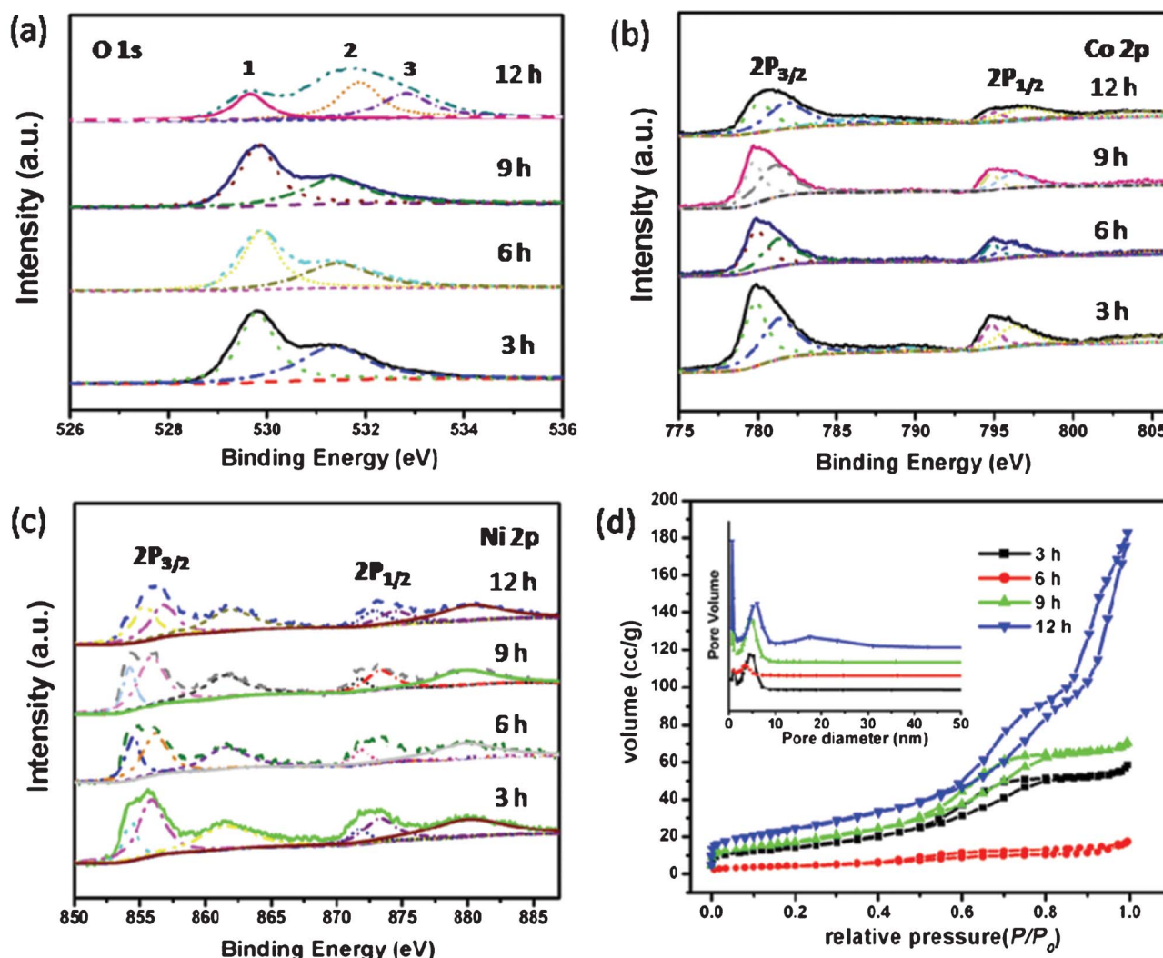
Fig. 6 (a–c) XPS spectra of \text{NiCo}_2\text{O}_4 samples at 180^\circ\text{C} from different hydrothermal reaction times; (d) \text{N}_2 adsorption/desorption isotherms of \text{NiCo}_2\text{O}_4 samples with corresponding pore-size distribution (inset).
