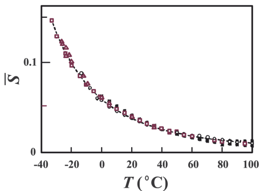
Fig. 8 Temperature dependence of \bar{S} (see the text for its definition) determined by the fitting of our predictions to the experimental data of \rho , K_T and C_p at various pressures. Open squares, triangles, and circles represent, respectively, data on \rho , K_T and C_p at ambient pressure. All the other symbols are data at higher pressures. The dashed line is our theoretical prediction for \bar{S} . The values of \bar{S} determined from the 23 sets of data of "bulk" liquid water are all collapsed on the master curve, which is described by the single Boltzmann factor. The figure is reproduced from Fig. 1(b) of ref. 21.
