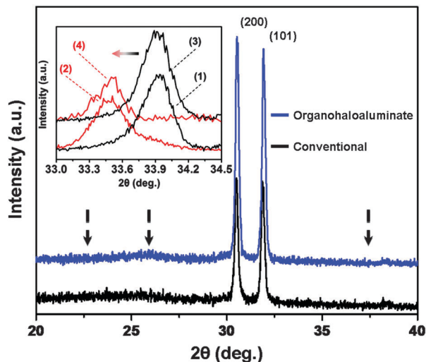
Fig. 4 XRD spectra of de-magnesiumated \text{Mg}_2\text{Sn} from organohaloaluminate (blue) and conventional (black) electrolytes ( \text{Mg}_2\text{Sn} peak positions marked with arrows). Inset – XRD spectra showing a peak shift due to magnesianation (red) of \text{Mo}_6\text{S}_8 (black) in organohaloaluminate (peak shift 1 \rightarrow 2) and conventional (peak shift 3 \rightarrow 4) electrolytes.
